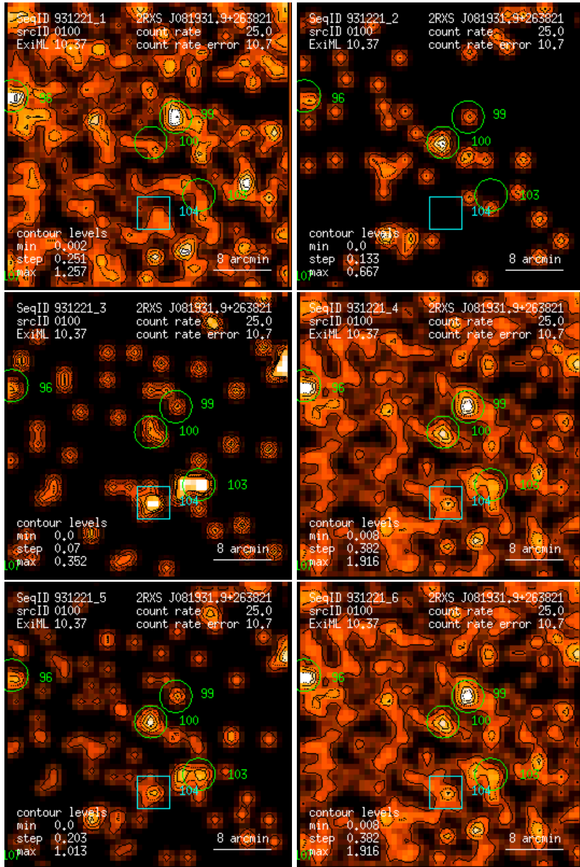
Figure 100: RASS 931221: detection 0100: band rate images, Gaussian filter: (1) PSPC channels 11 – 41, (2) 52 – 90, (3) 91 – 201, (4) 11 – 235, (5) 52 – 201, (6) 11 – 201. Broad band rates in counts/ks. Band rate contour levels in counts/ks/arcmin 2 .
