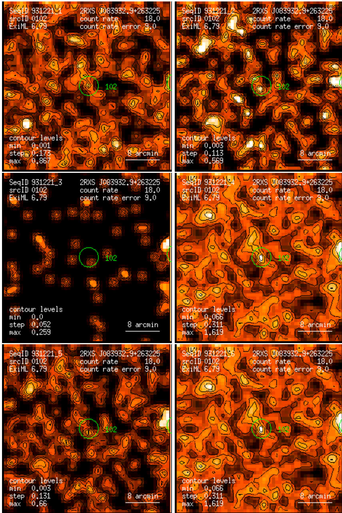
Figure 102: RASS 931221: detection 0102: band rate images, Gaussian filter: (1) PSPC channels 11 – 41, (2) 52 – 90, (3) 91 – 201, (4) 11 – 235, (5) 52 – 201, (6) 11 – 201. Broad band rates in counts/ks. Band rate contour levels in counts/ks/arcmin 2 .
