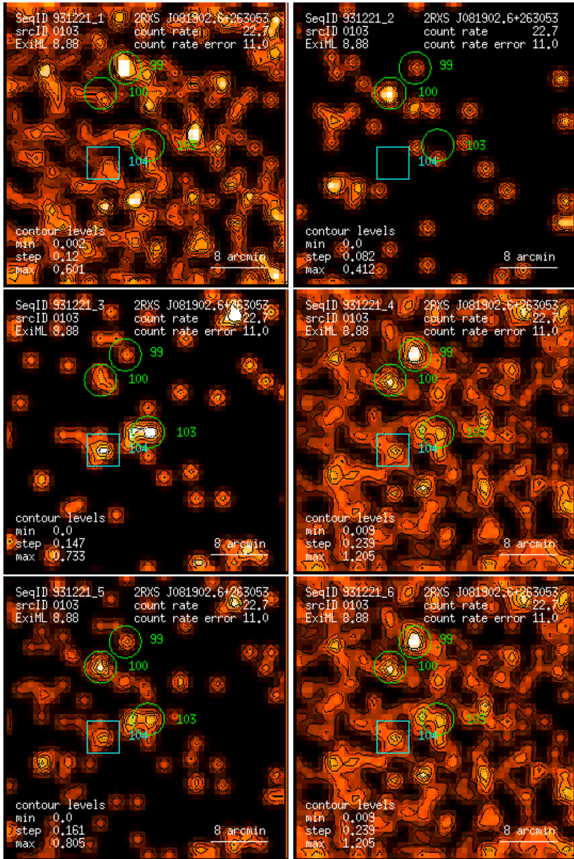
Figure 103: RASS 931221: detection 0103: band rate images, Gaussian filter: (1) PSPC channels 11 – 41, (2) 52 – 90, (3) 91 – 201, (4) 11 – 235, (5) 52 – 201, (6) 11 – 201. Broad band rates in counts/ks. Band rate contour levels in counts/ks/arcmin 2 .
