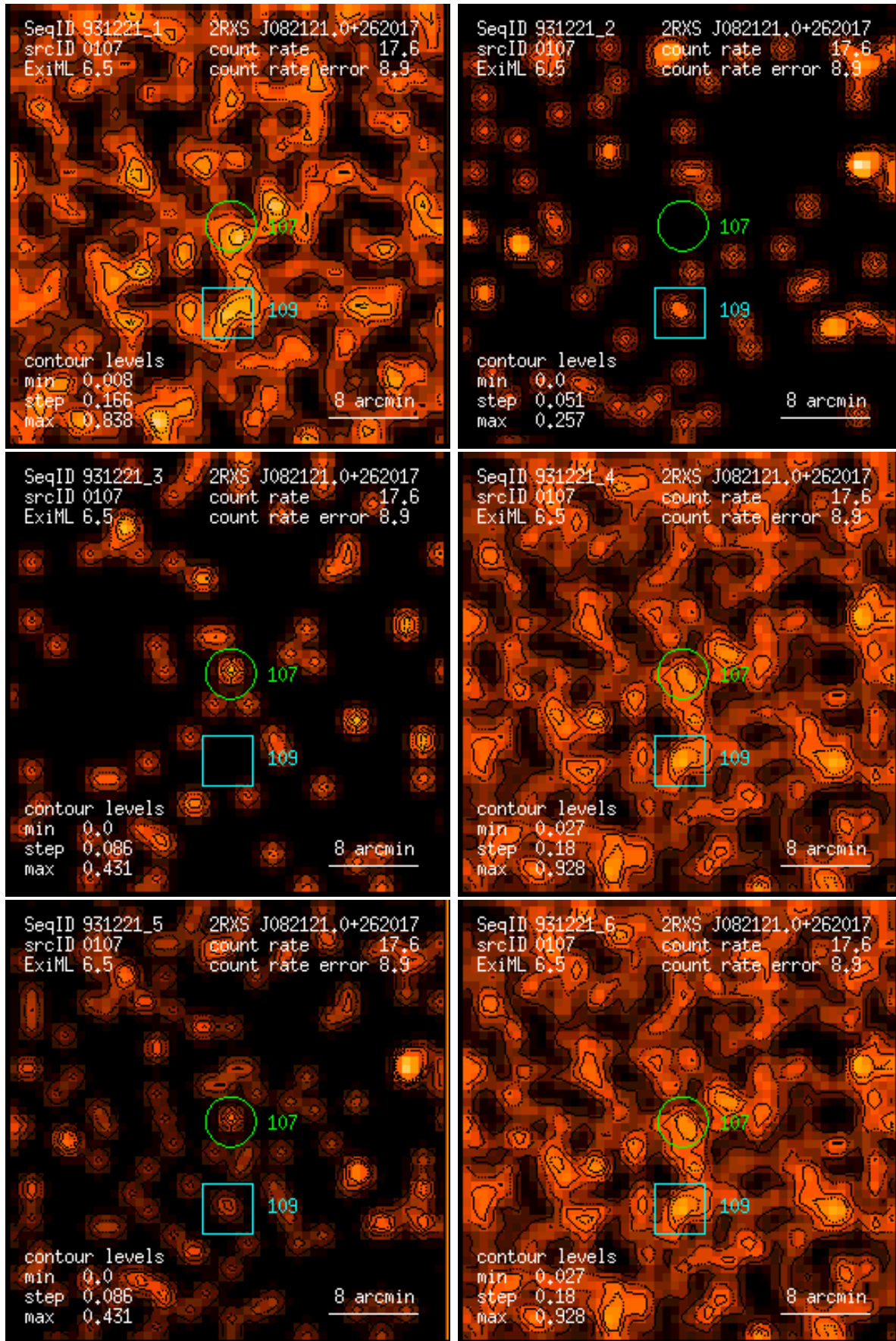
Figure 107: RASS 931221: detection 0107: band rate images, Gaussian filter: (1) PSPC channels 11 – 41, (2) 52 – 90, (3) 91 – 201, (4) 11 – 235, (5) 52 – 201, (6) 11 – 201. Broad band rates in counts/ks. Band rate contour levels in counts/ks/arcmin 2 .
