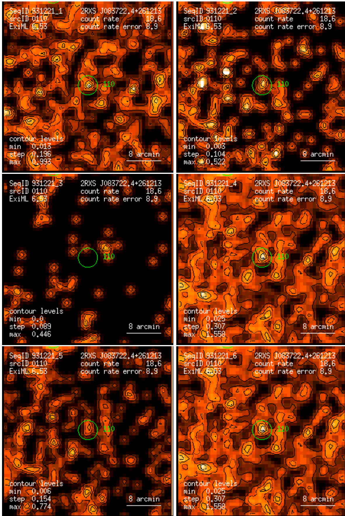
Figure 110: RASS 931221: detection 0110: band rate images, Gaussian filter: (1) PSPC channels 11 – 41, (2) 52 – 90, (3) 91 – 201, (4) 11 – 235, (5) 52 – 201, (6) 11 – 201. Broad band rates in counts/ks. Band rate contour levels in counts/ks/arcmin 2 .
