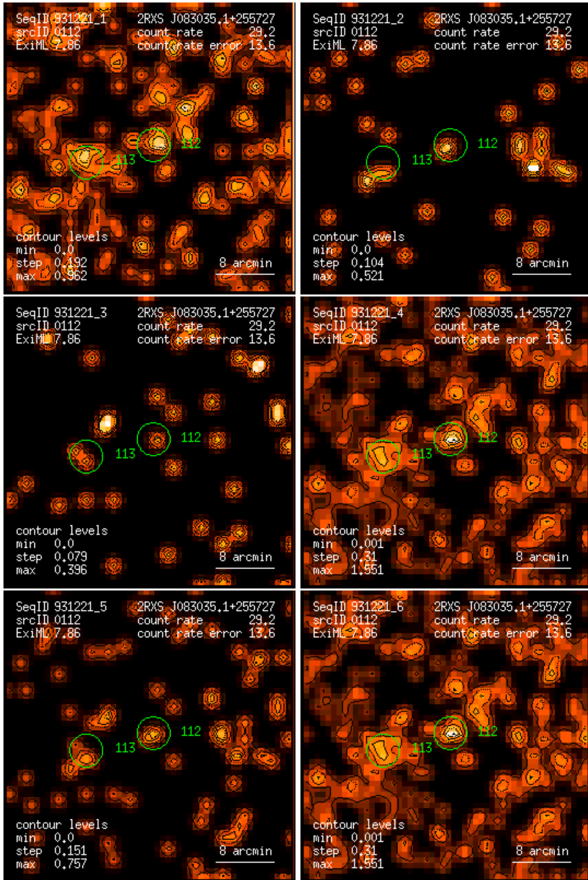
Figure 112: RASS 931221: detection 0112: band rate images, Gaussian filter: (1) PSPC channels 11 – 41, (2) 52 – 90, (3) 91 – 201, (4) 11 – 235, (5) 52 – 201, (6) 11 – 201. Broad band rates in counts/ks. Band rate contour levels in counts/ks/arcmin 2 .
