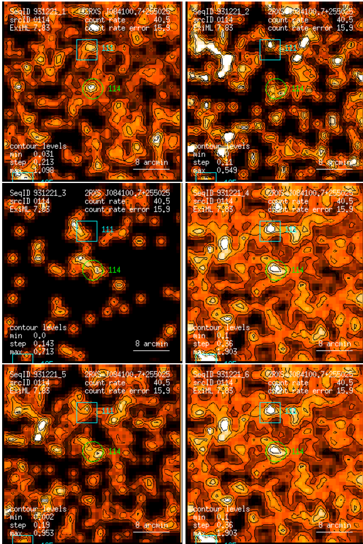
Figure 114: RASS 931221: detection 0114: band rate images, Gaussian filter: (1) PSPC channels 11 – 41, (2) 52 – 90, (3) 91 – 201, (4) 11 – 235, (5) 52 – 201, (6) 11 – 201. Broad band rates in counts/ks. Band rate contour levels in counts/ks/arcmin 2 .
