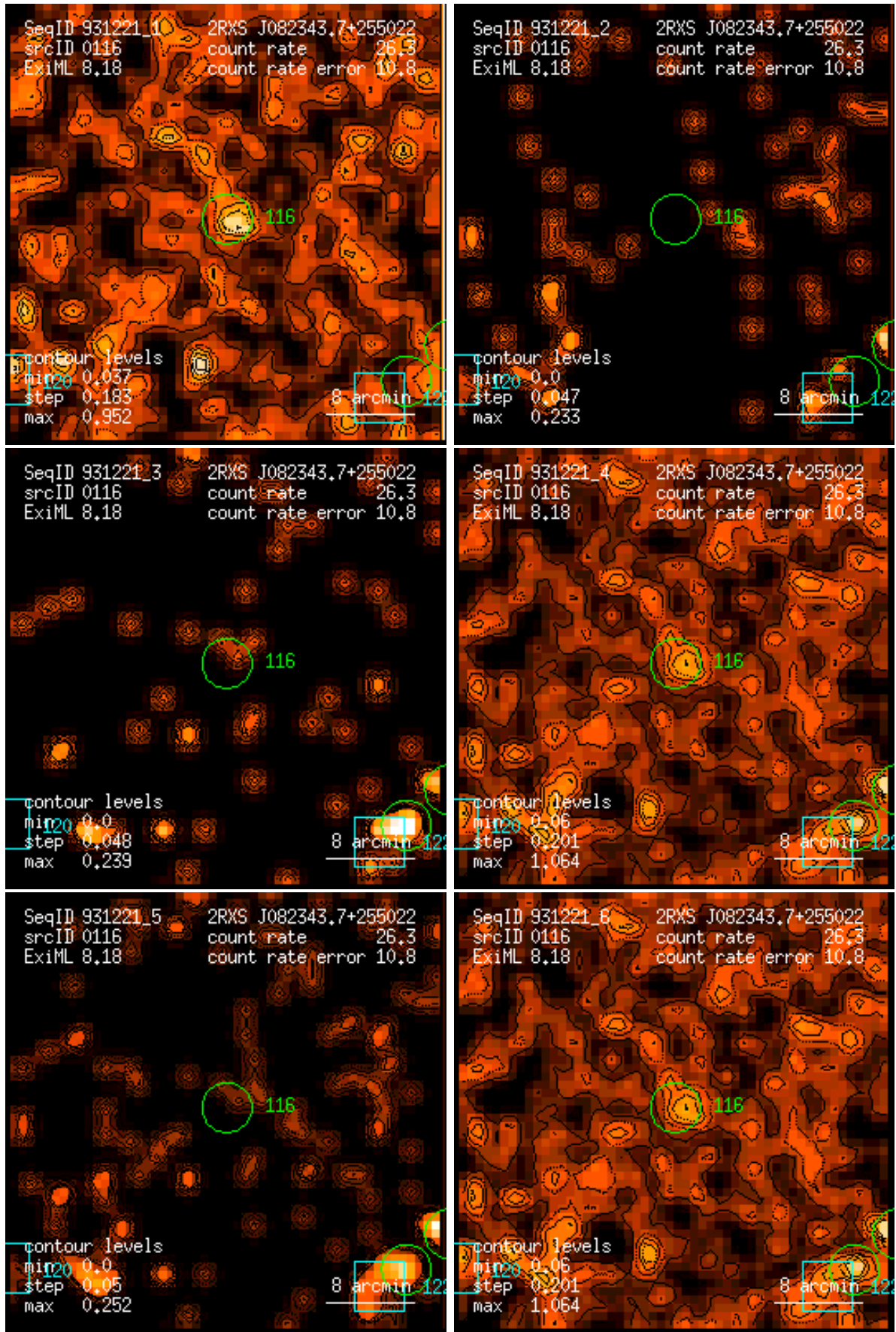
Figure 116: RASS 931221: detection 0116: band rate images, Gaussian filter: (1) PSPC channels 11 – 41, (2) 52 – 90, (3) 91 – 201, (4) 11 – 235, (5) 52 – 201, (6) 11 – 201. Broad band rates in counts/ks. Band rate contour levels in counts/ks/arcmin 2 .
