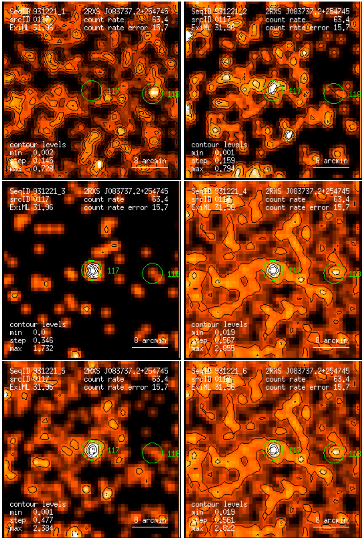
Figure 117: RASS 931221: detection 0117: band rate images, Gaussian filter: (1) PSPC channels 11 – 41, (2) 52 – 90, (3) 91 – 201, (4) 11 – 235, (5) 52 – 201, (6) 11 – 201. Broad band rates in counts/ks. Band rate contour levels in counts/ks/arcmin 2 .
