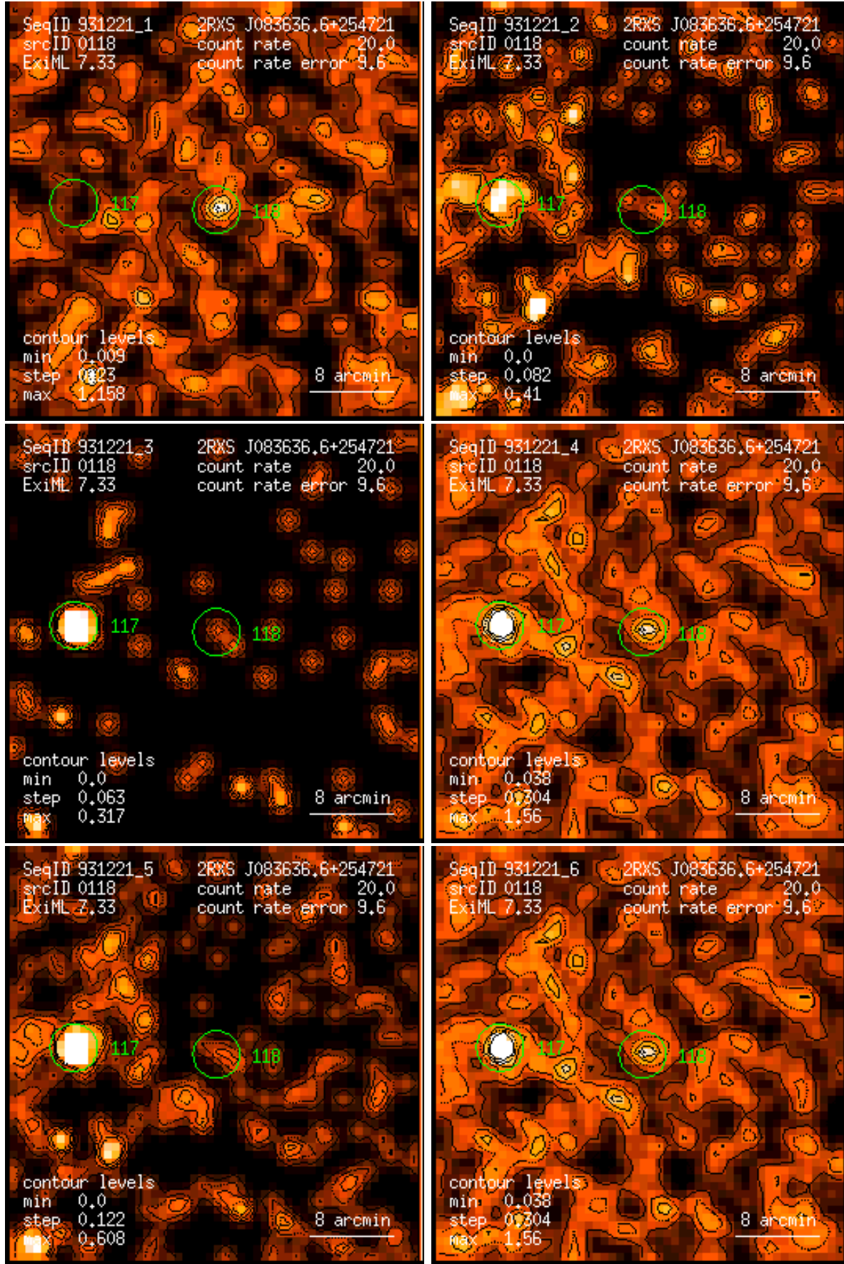
Figure 118: RASS 931221: detection 0118: band rate images, Gaussian filter: (1) PSPC channels 11 – 41, (2) 52 – 90, (3) 91 – 201, (4) 11 – 235, (5) 52 – 201, (6) 11 – 201. Broad band rates in counts/ks. Band rate contour levels in counts/ks/arcmin 2 .
