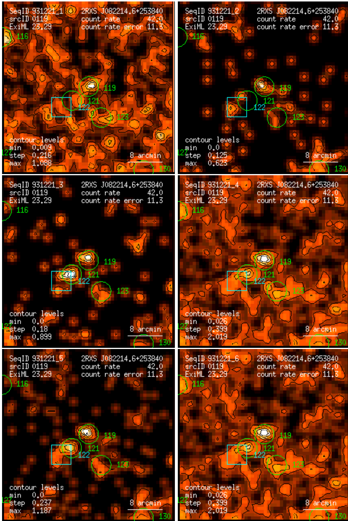
Figure 119: RASS 931221: detection 0119: band rate images, Gaussian filter: (1) PSPC channels 11 – 41, (2) 52 – 90, (3) 91 – 201, (4) 11 – 235, (5) 52 – 201, (6) 11 – 201. Broad band rates in counts/ks. Band rate contour levels in counts/ks/arcmin 2 .
