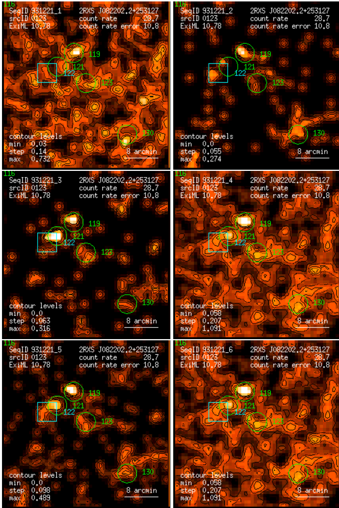
Figure 123: RASS 931221: detection 0123: band rate images, Gaussian filter: (1) PSPC channels 11 – 41, (2) 52 – 90, (3) 91 – 201, (4) 11 – 235, (5) 52 – 201, (6) 11 – 201. Broad band rates in counts/ks. Band rate contour levels in counts/ks/arcmin 2 .
