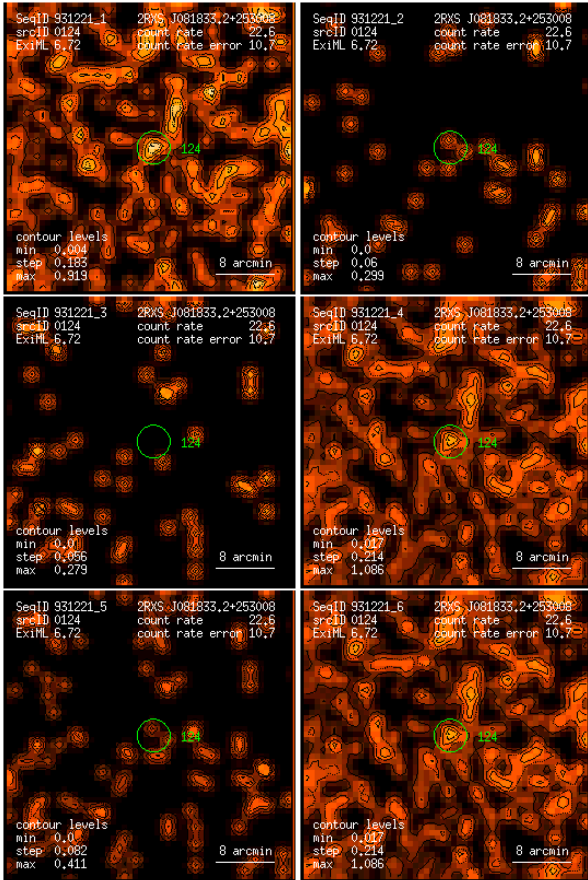
Figure 124: RASS 931221: detection 0124: band rate images, Gaussian filter: (1) PSPC channels 11 – 41, (2) 52 – 90, (3) 91 – 201, (4) 11 – 235, (5) 52 – 201, (6) 11 – 201. Broad band rates in counts/ks. Band rate contour levels in counts/ks/arcmin 2 .
