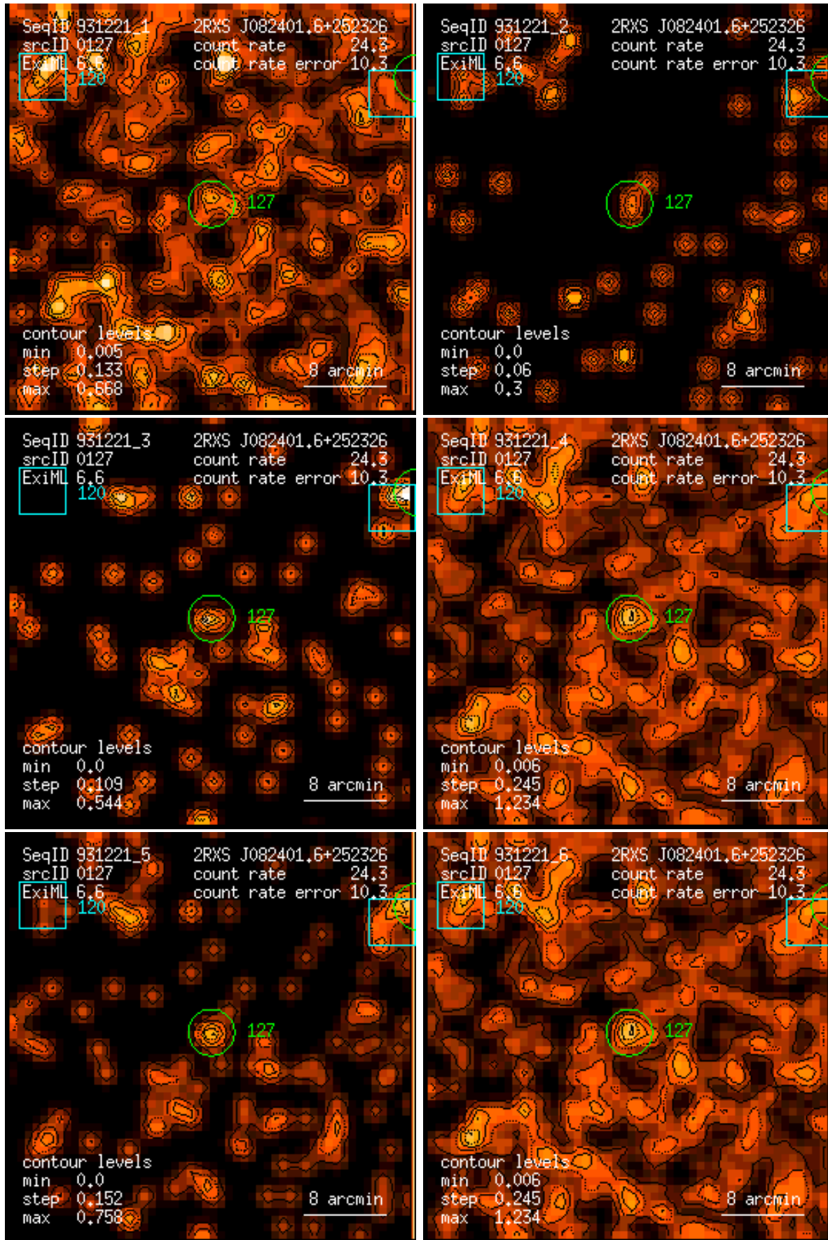
Figure 127: RASS 931221: detection 0127: band rate images, Gaussian filter: (1) PSPC channels 11 – 41, (2) 52 – 90, (3) 91 – 201, (4) 11 – 235, (5) 52 – 201, (6) 11 – 201. Broad band rates in counts/ks. Band rate contour levels in counts/ks/arcmin 2 .
