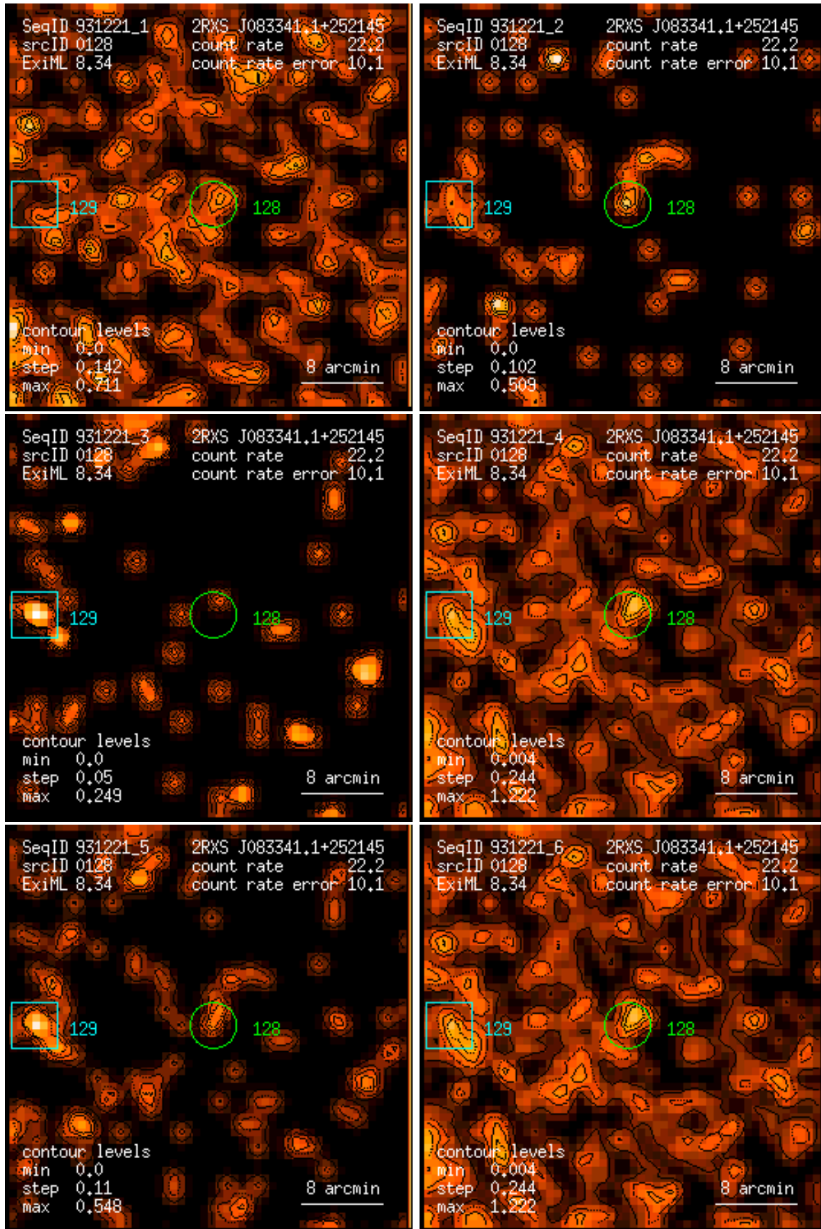
Figure 128: RASS 931221: detection 0128: band rate images, Gaussian filter: (1) PSPC channels 11 – 41, (2) 52 – 90, (3) 91 – 201, (4) 11 – 235, (5) 52 – 201, (6) 11 – 201. Broad band rates in counts/ks. Band rate contour levels in counts/ks/arcmin 2 .
