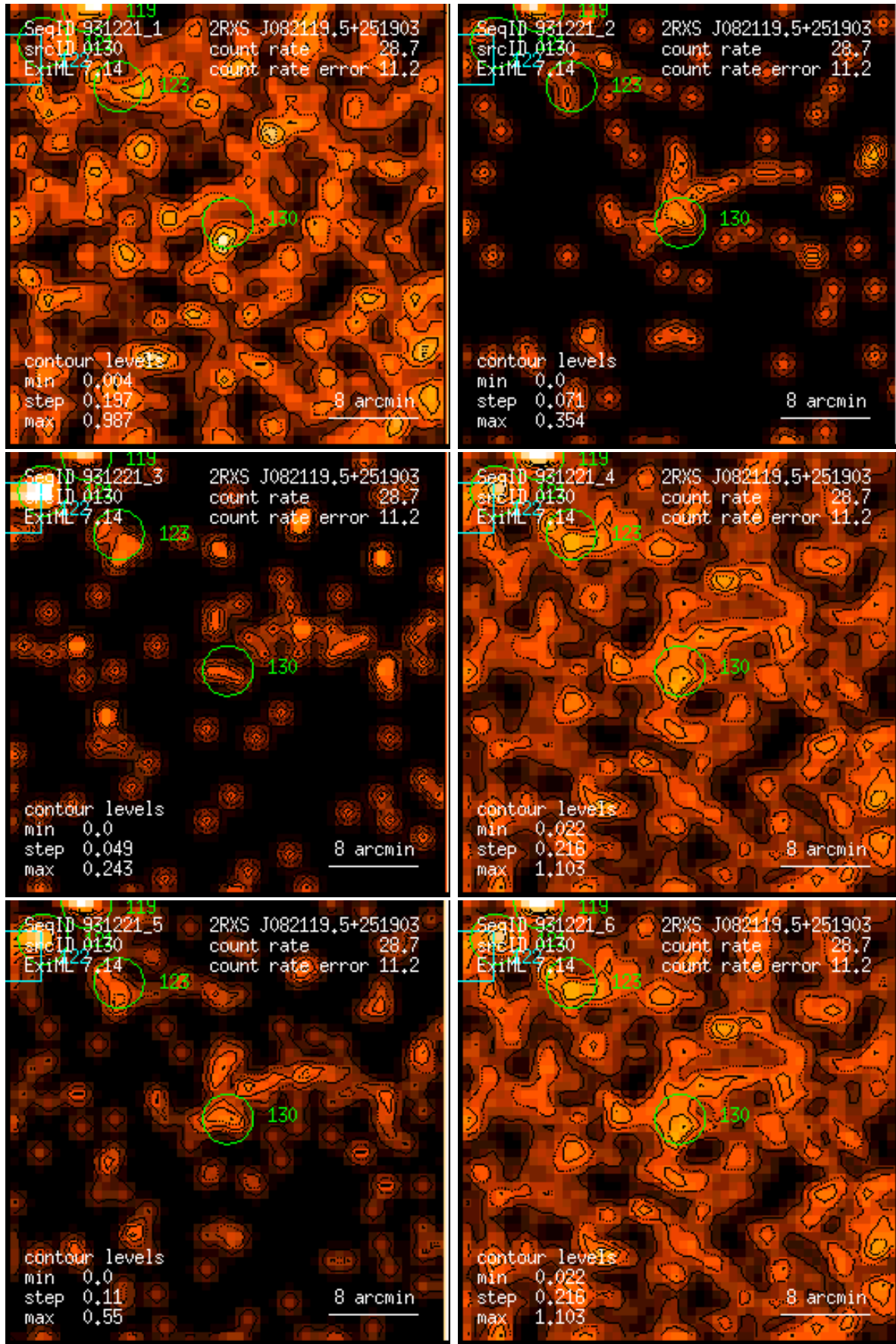
Figure 130: RASS 931221: detection 0130: band rate images, Gaussian filter: (1) PSPC channels 11 – 41, (2) 52 – 90, (3) 91 – 201, (4) 11 – 235, (5) 52 – 201, (6) 11 – 201. Broad band rates in counts/ks. Band rate contour levels in counts/ks/arcmin 2 .
