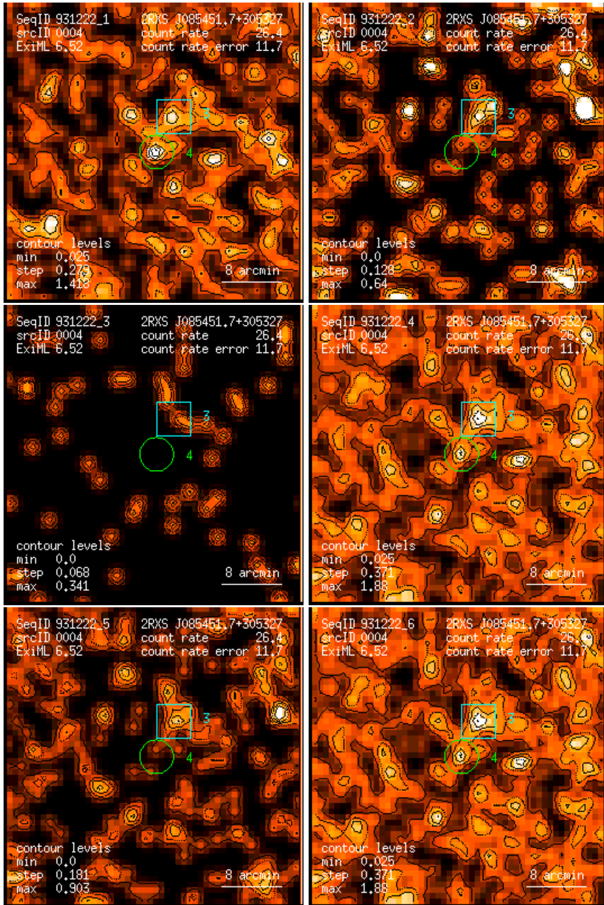
Figure 4: RASS 931222: detection 0004: band rate images, Gaussian filter: (1) PSPC channels 11 – 41, (2) 52 – 90, (3) 91 – 201, (4) 11 – 235, (5) 52 – 201, (6) 11 – 201. Broad band rates in counts/ks. Band rate contour levels in counts/ks/arcmin 2 .
