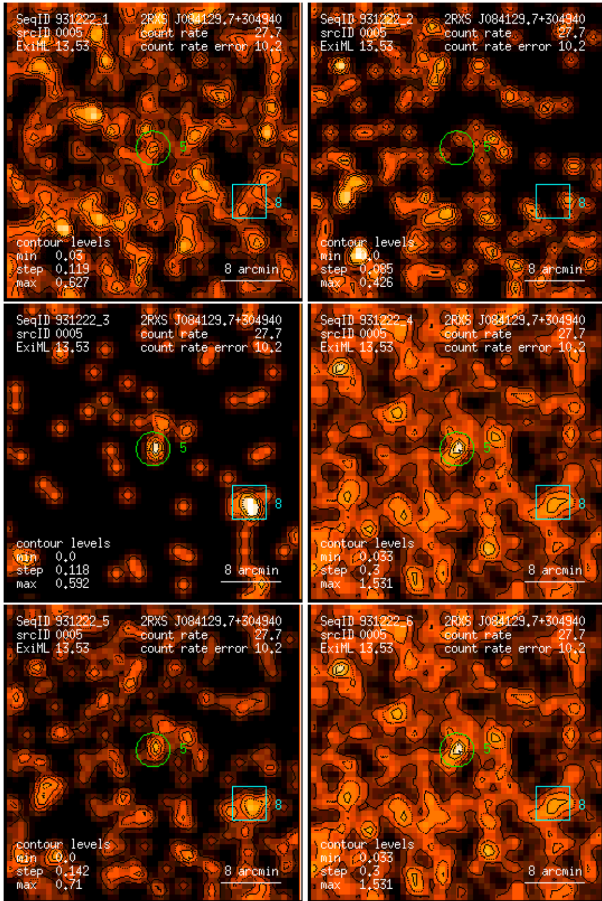
Figure 5: RASS 931222: detection 0005: band rate images, Gaussian filter: (1) PSPC channels 11 – 41, (2) 52 – 90, (3) 91 – 201, (4) 11 – 235, (5) 52 – 201, (6) 11 – 201. Broad band rates in counts/ks. Band rate contour levels in counts/ks/arcmin 2 .
