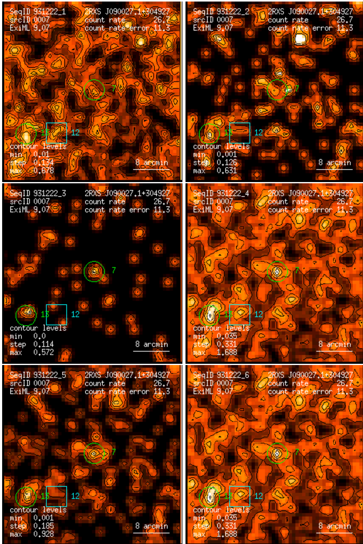
Figure 7: RASS 931222: detection 0007: band rate images, Gaussian filter: (1) PSPC channels 11 – 41, (2) 52 – 90, (3) 91 – 201, (4) 11 – 235, (5) 52 – 201, (6) 11 – 201. Broad band rates in counts/ks. Band rate contour levels in counts/ks/arcmin 2 .
