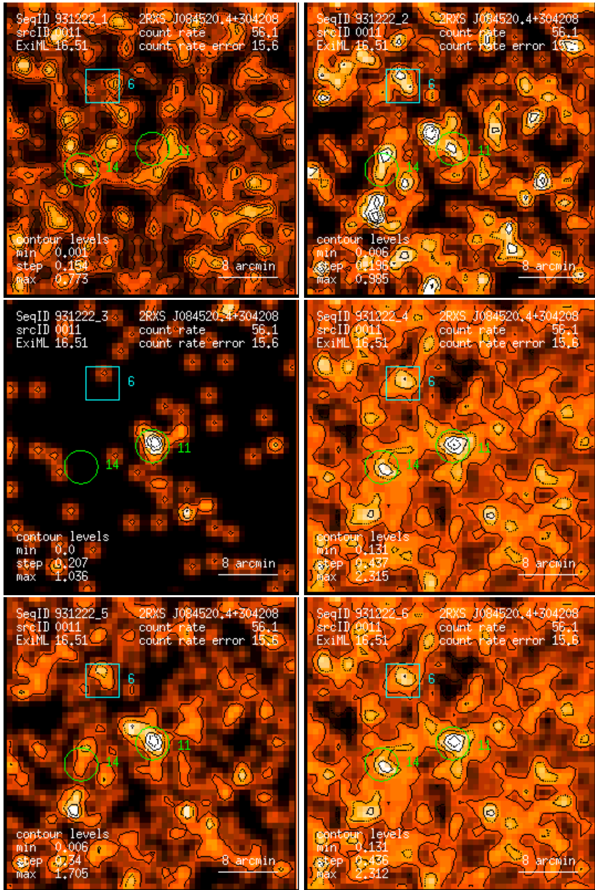
Figure 11: RASS 931222: detection 0011: band rate images, Gaussian filter: (1) PSPC channels 11 – 41, (2) 52 – 90, (3) 91 – 201, (4) 11 – 235, (5) 52 – 201, (6) 11 – 201. Broad band rates in counts/ks. Band rate contour levels in counts/ks/arcmin 2 .
