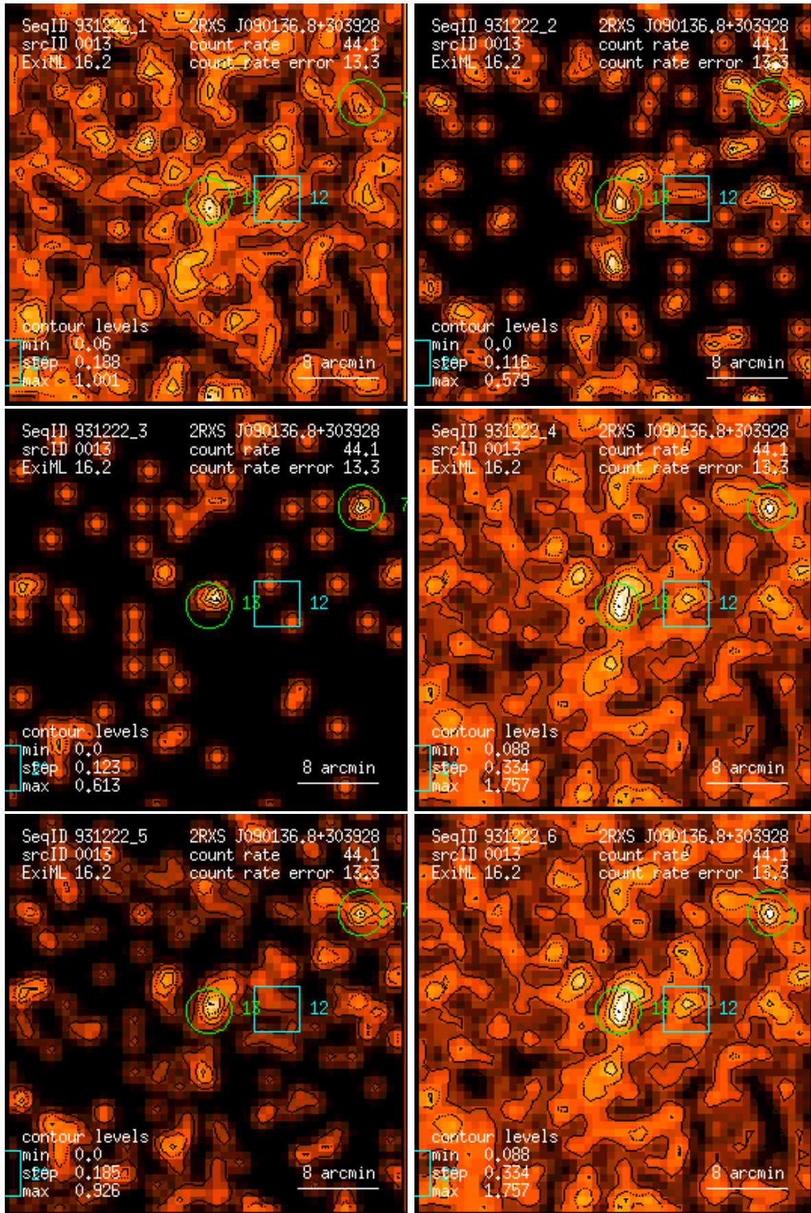
Figure 13: RASS 931222: detection 0013: band rate images, Gaussian filter: (1) PSPC channels 11 – 41, (2) 52 – 90, (3) 91 – 201, (4) 11 – 235, (5) 52 – 201, (6) 11 – 201. Broad band rates in counts/ks. Band rate contour levels in counts/ks/arcmin 2 .
