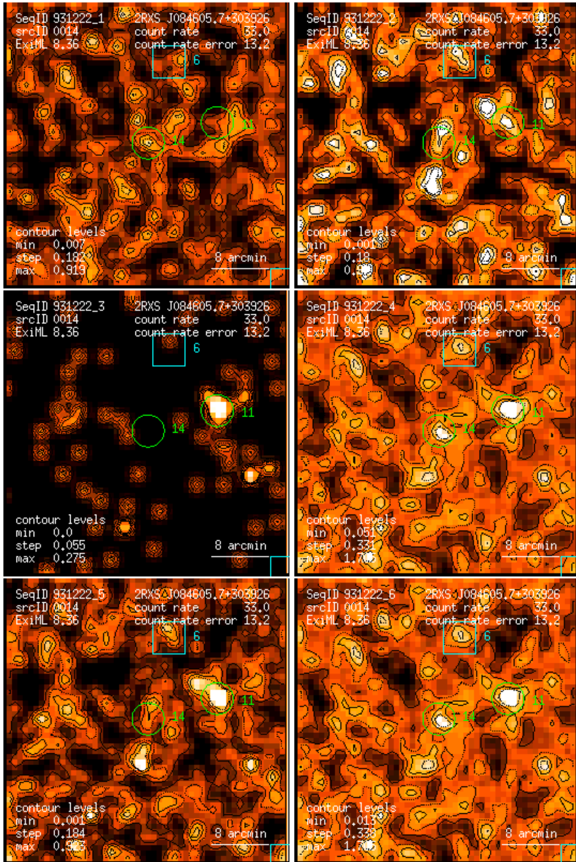
Figure 14: RASS 931222: detection 0014: band rate images, Gaussian filter: (1) PSPC channels 11 – 41, (2) 52 – 90, (3) 91 – 201, (4) 11 – 235, (5) 52 – 201, (6) 11 – 201. Broad band rates in counts/ks. Band rate contour levels in counts/ks/arcmin 2 .
