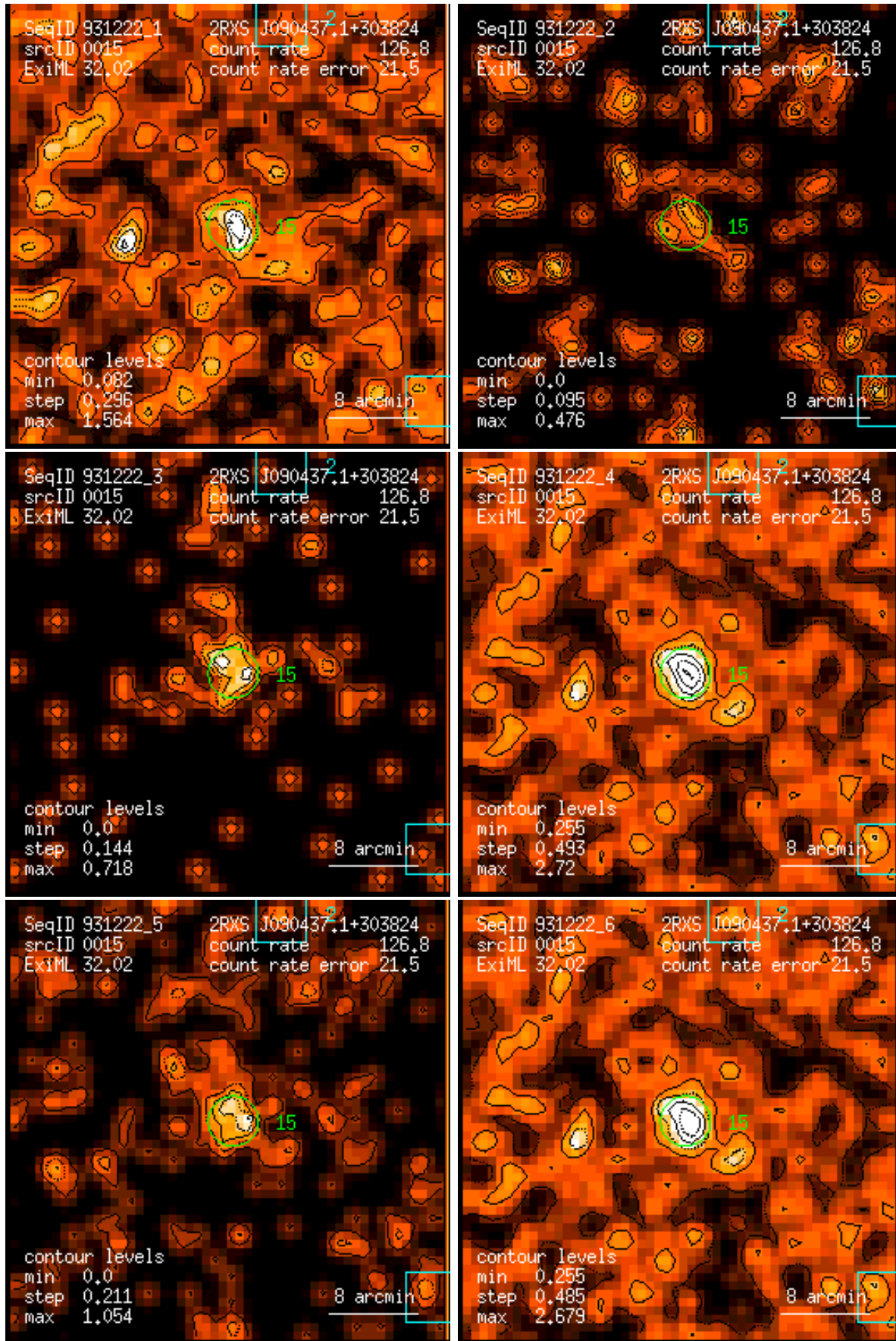
Figure 15: RASS 931222: detection 0015: band rate images, Gaussian filter: (1) PSPC channels 11 – 41, (2) 52 – 90, (3) 91 – 201, (4) 11 – 235, (5) 52 – 201, (6) 11 – 201. Broad band rates in counts/ks. Band rate contour levels in counts/ks/arcmin 2 .
