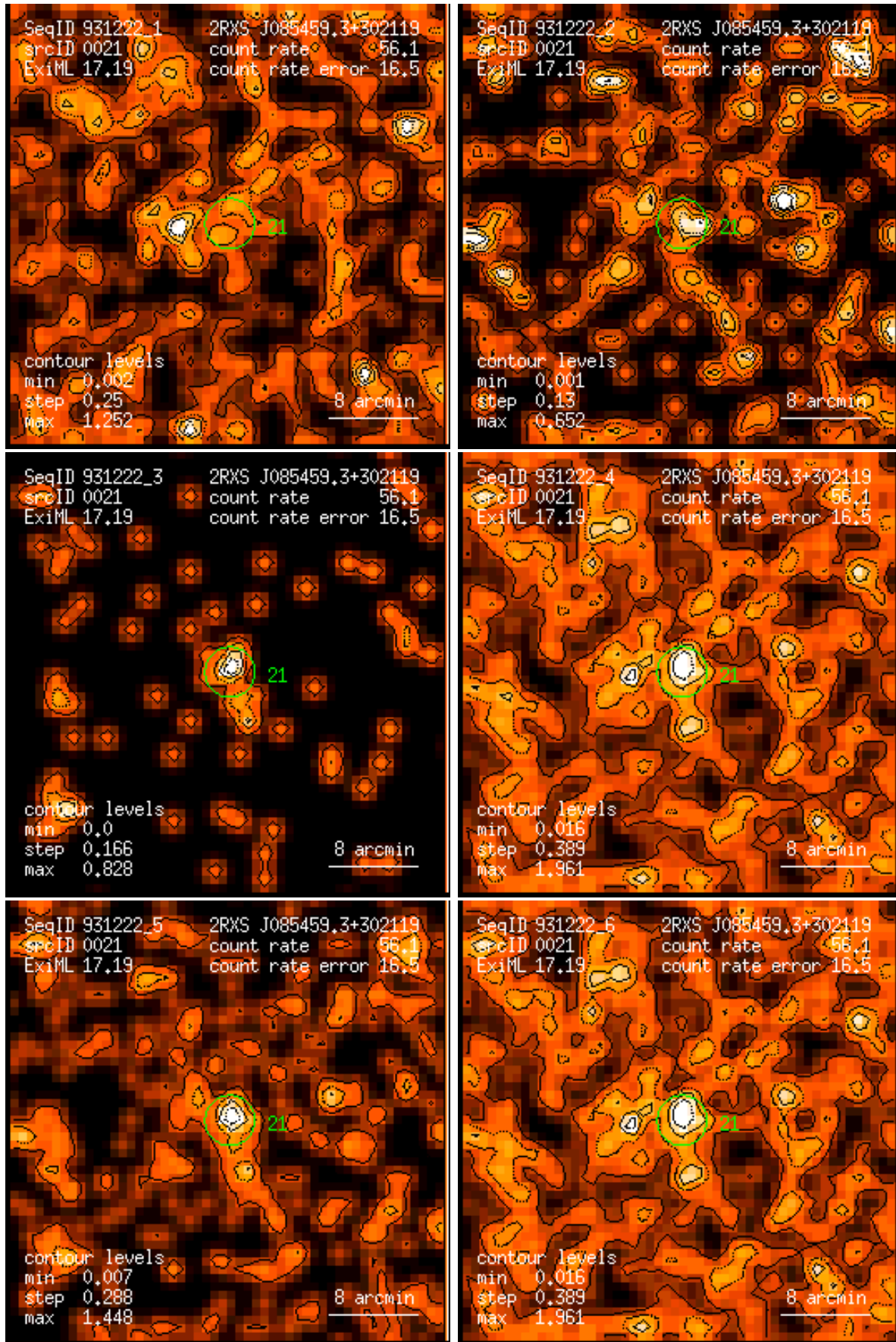
Figure 21: RASS 931222: detection 0021: band rate images, Gaussian filter: (1) PSPC channels 11 – 41, (2) 52 – 90, (3) 91 – 201, (4) 11 – 235, (5) 52 – 201, (6) 11 – 201. Broad band rates in counts/ks. Band rate contour levels in counts/ks/arcmin 2 .
