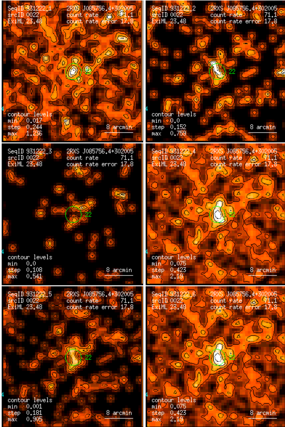
Figure 22: RASS 931222: detection 0022: band rate images, Gaussian filter: (1) PSPC channels 11 – 41, (2) 52 – 90, (3) 91 – 201, (4) 11 – 235, (5) 52 – 201, (6) 11 – 201. Broad band rates in counts/ks. Band rate contour levels in counts/ks/arcmin 2 .
