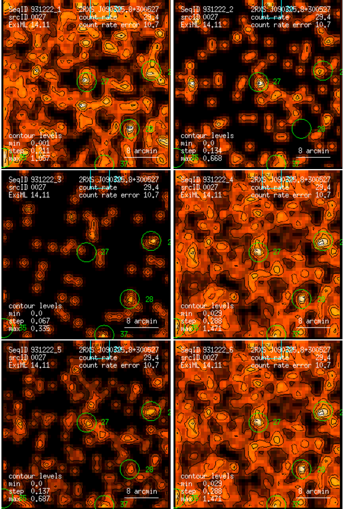
Figure 27: RASS 931222: detection 0027: band rate images, Gaussian filter: (1) PSPC channels 11 – 41, (2) 52 – 90, (3) 91 – 201, (4) 11 – 235, (5) 52 – 201, (6) 11 – 201. Broad band rates in counts/ks. Band rate contour levels in counts/ks/arcmin 2 .
