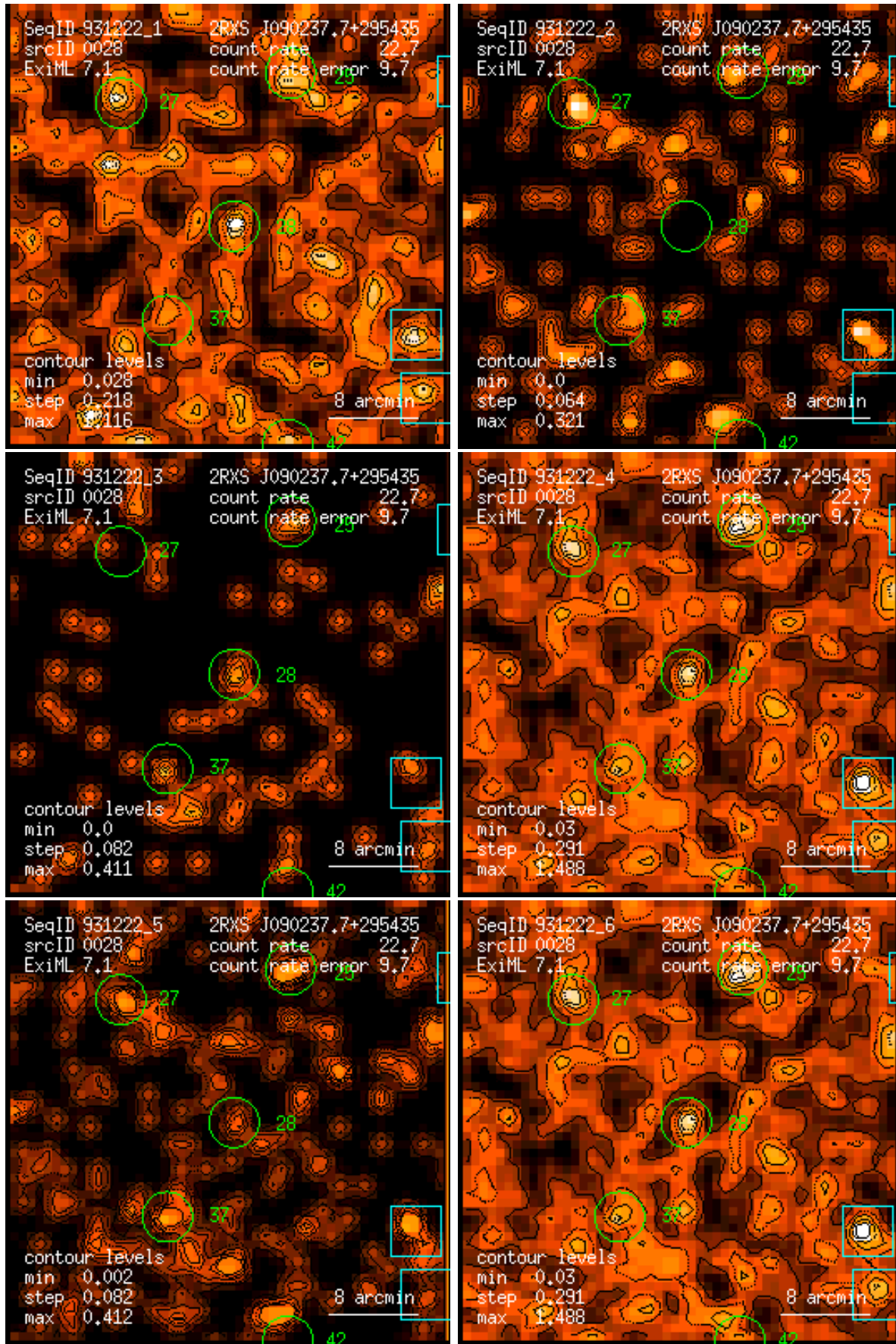
Figure 28: RASS 931222: detection 0028: band rate images, Gaussian filter: (1) PSPC channels 11 – 41, (2) 52 – 90, (3) 91 – 201, (4) 11 – 235, (5) 52 – 201, (6) 11 – 201. Broad band rates in counts/ks. Band rate contour levels in counts/ks/arcmin 2 .
