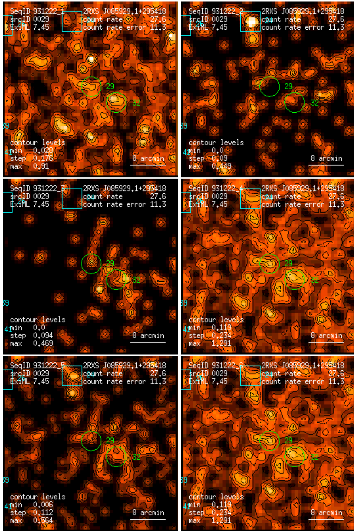
Figure 29: RASS 931222: detection 0029: band rate images, Gaussian filter: (1) PSPC channels 11 – 41, (2) 52 – 90, (3) 91 – 201, (4) 11 – 235, (5) 52 – 201, (6) 11 – 201. Broad band rates in counts/ks. Band rate contour levels in counts/ks/arcmin 2 .
