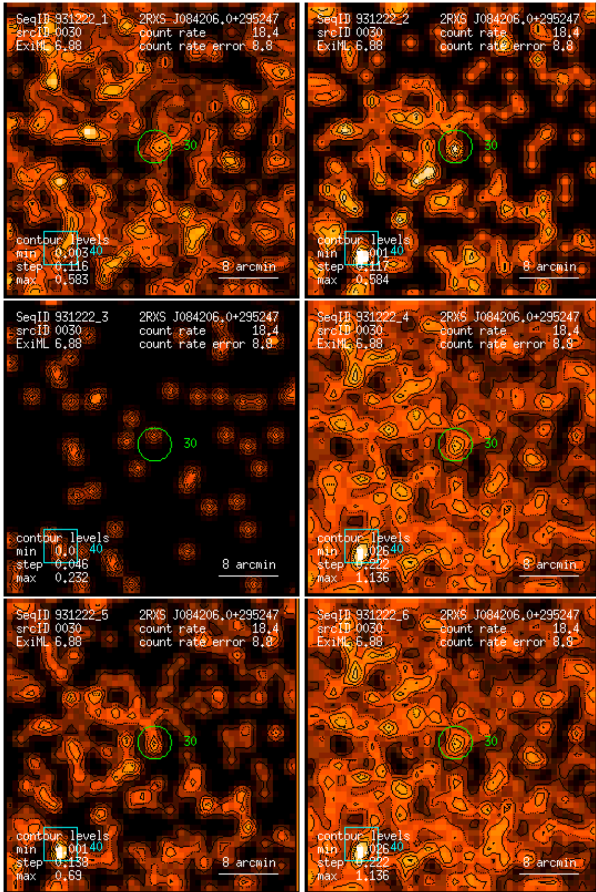
Figure 30: RASS 931222: detection 0030: band rate images, Gaussian filter: (1) PSPC channels 11 – 41, (2) 52 – 90, (3) 91 – 201, (4) 11 – 235, (5) 52 – 201, (6) 11 – 201. Broad band rates in counts/ks. Band rate contour levels in counts/ks/arcmin 2 .
