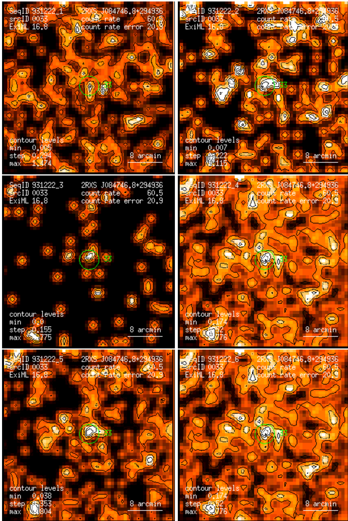
Figure 33: RASS 931222: detection 0033: band rate images, Gaussian filter: (1) PSPC channels 11 – 41, (2) 52 – 90, (3) 91 – 201, (4) 11 – 235, (5) 52 – 201, (6) 11 – 201. Broad band rates in counts/ks. Band rate contour levels in counts/ks/arcmin 2 .
