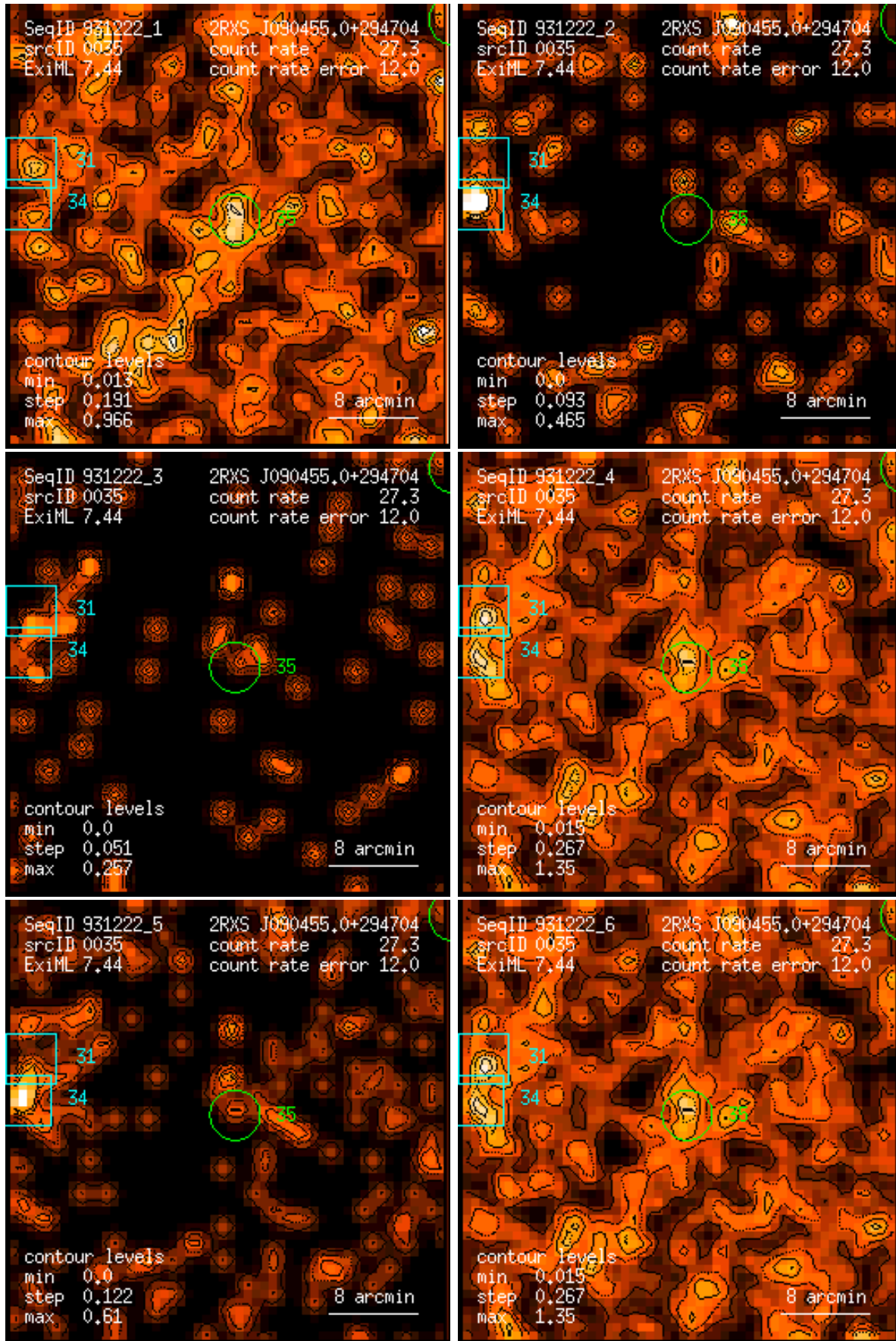
Figure 35: RASS 931222: detection 0035: band rate images, Gaussian filter: (1) PSPC channels 11 – 41, (2) 52 – 90, (3) 91 – 201, (4) 11 – 235, (5) 52 – 201, (6) 11 – 201. Broad band rates in counts/ks. Band rate contour levels in counts/ks/arcmin 2 .
