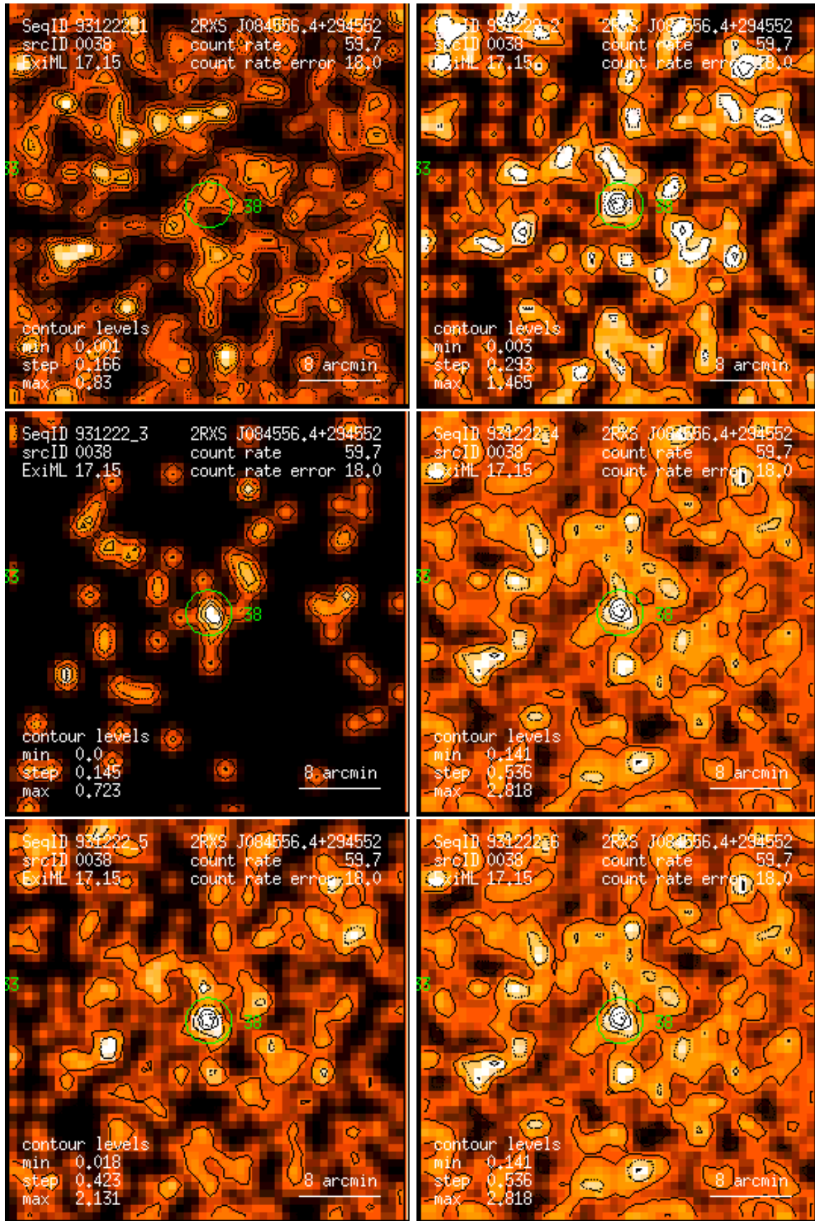
Figure 38: RASS 931222: detection 0038: band rate images, Gaussian filter: (1) PSPC channels 11 – 41, (2) 52 – 90, (3) 91 – 201, (4) 11 – 235, (5) 52 – 201, (6) 11 – 201. Broad band rates in counts/ks. Band rate contour levels in counts/ks/arcmin 2 .
