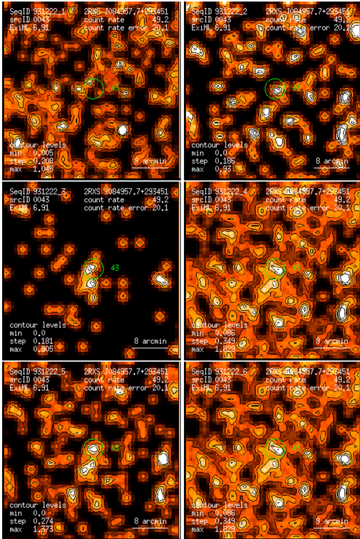
Figure 43: RASS 931222: detection 0043: band rate images, Gaussian filter: (1) PSPC channels 11 – 41, (2) 52 – 90, (3) 91 – 201, (4) 11 – 235, (5) 52 – 201, (6) 11 – 201. Broad band rates in counts/ks. Band rate contour levels in counts/ks/arcmin 2 .
