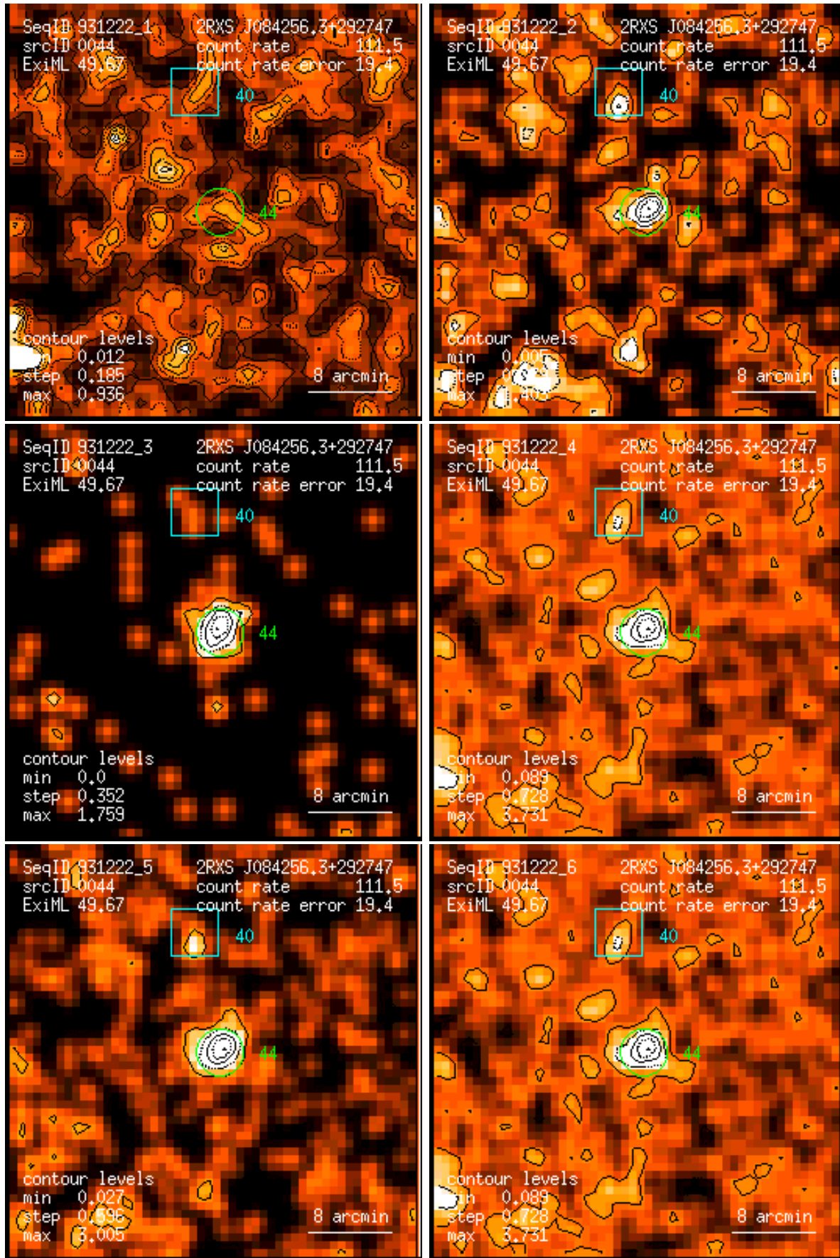
Figure 44: RASS 931222: detection 0044: band rate images, Gaussian filter: (1) PSPC channels 11 – 41, (2) 52 – 90, (3) 91 – 201, (4) 11 – 235, (5) 52 – 201, (6) 11 – 201. Broad band rates in counts/ks. Band rate contour levels in counts/ks/arcmin 2 .
