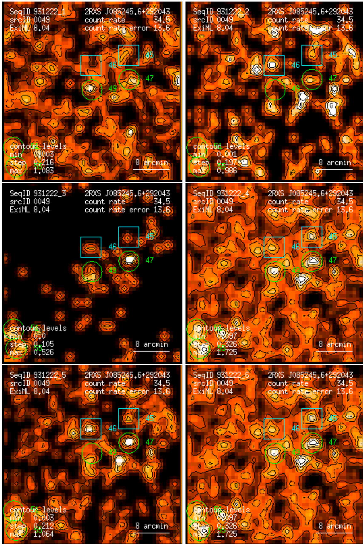
Figure 49: RASS 931222: detection 0049: band rate images, Gaussian filter: (1) PSPC channels 11 – 41, (2) 52 – 90, (3) 91 – 201, (4) 11 – 235, (5) 52 – 201, (6) 11 – 201. Broad band rates in counts/ks. Band rate contour levels in counts/ks/arcmin 2 .
