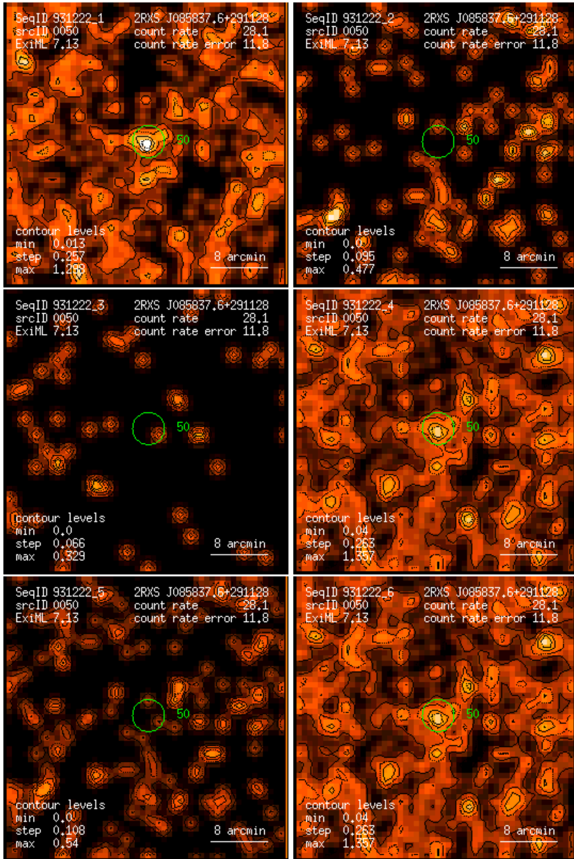
Figure 50: RASS 931222: detection 0050: band rate images, Gaussian filter: (1) PSPC channels 11 – 41, (2) 52 – 90, (3) 91 – 201, (4) 11 – 235, (5) 52 – 201, (6) 11 – 201. Broad band rates in counts/ks. Band rate contour levels in counts/ks/arcmin 2 .
