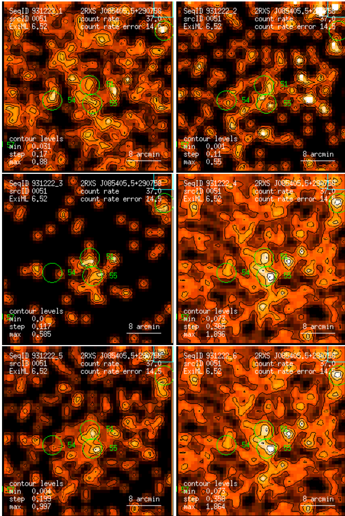
Figure 51: RASS 931222: detection 0051: band rate images, Gaussian filter: (1) PSPC channels 11 – 41, (2) 52 – 90, (3) 91 – 201, (4) 11 – 235, (5) 52 – 201, (6) 11 – 201. Broad band rates in counts/ks. Band rate contour levels in counts/ks/arcmin 2 .
