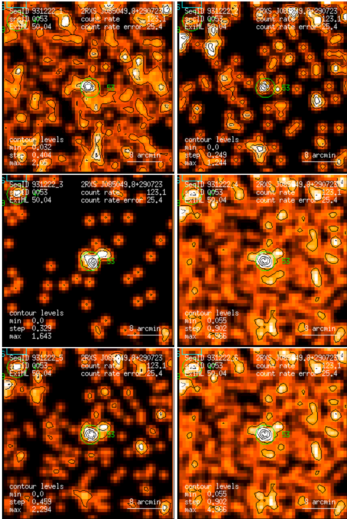
Figure 53: RASS 931222: detection 0053: band rate images, Gaussian filter: (1) PSPC channels 11 – 41, (2) 52 – 90, (3) 91 – 201, (4) 11 – 235, (5) 52 – 201, (6) 11 – 201. Broad band rates in counts/ks. Band rate contour levels in counts/ks/arcmin 2 .
