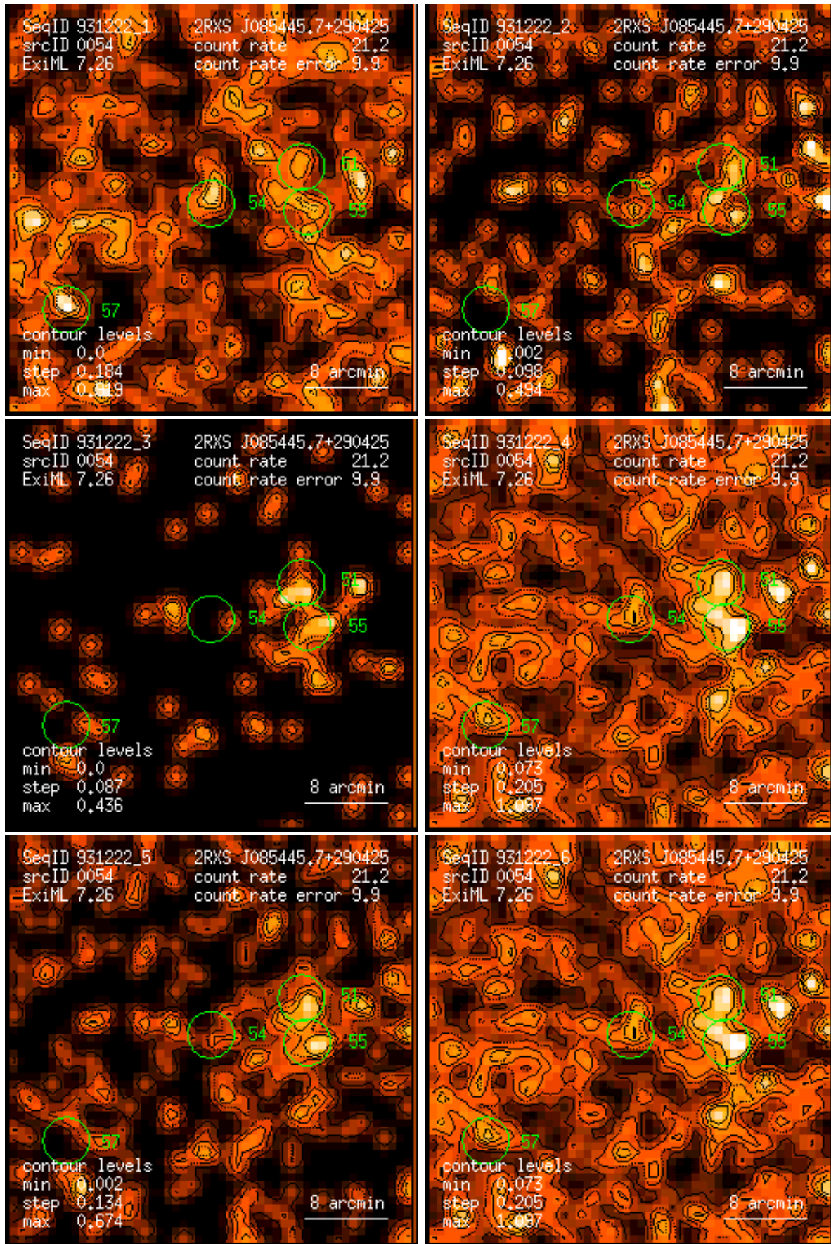
Figure 54: RASS 931222: detection 0054: band rate images, Gaussian filter: (1) PSPC channels 11 – 41, (2) 52 – 90, (3) 91 – 201, (4) 11 – 235, (5) 52 – 201, (6) 11 – 201. Broad band rates in counts/ks. Band rate contour levels in counts/ks/arcmin 2 .
