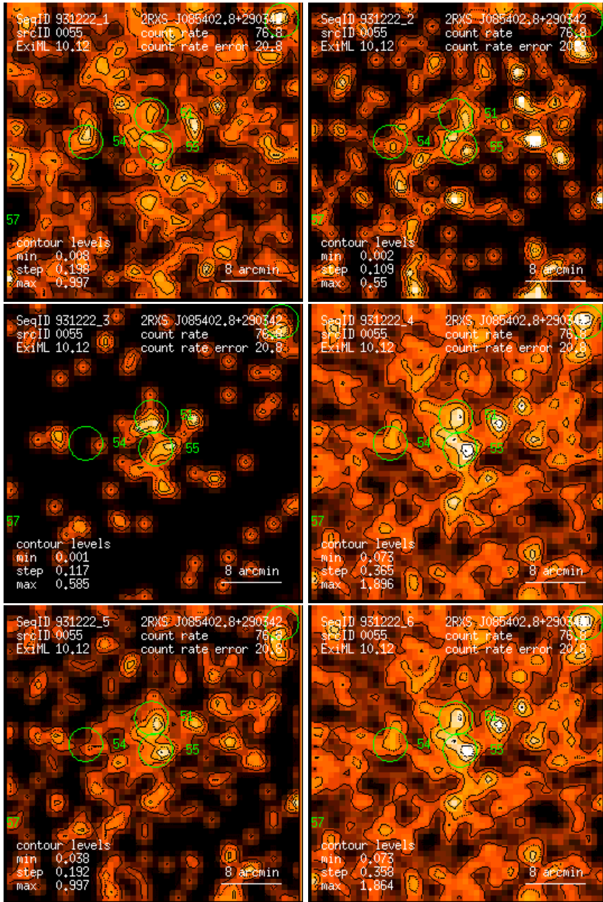
Figure 55: RASS 931222: detection 0055: band rate images, Gaussian filter: (1) PSPC channels 11 – 41, (2) 52 – 90, (3) 91 – 201, (4) 11 – 235, (5) 52 – 201, (6) 11 – 201. Broad band rates in counts/ks. Band rate contour levels in counts/ks/arcmin 2 .
