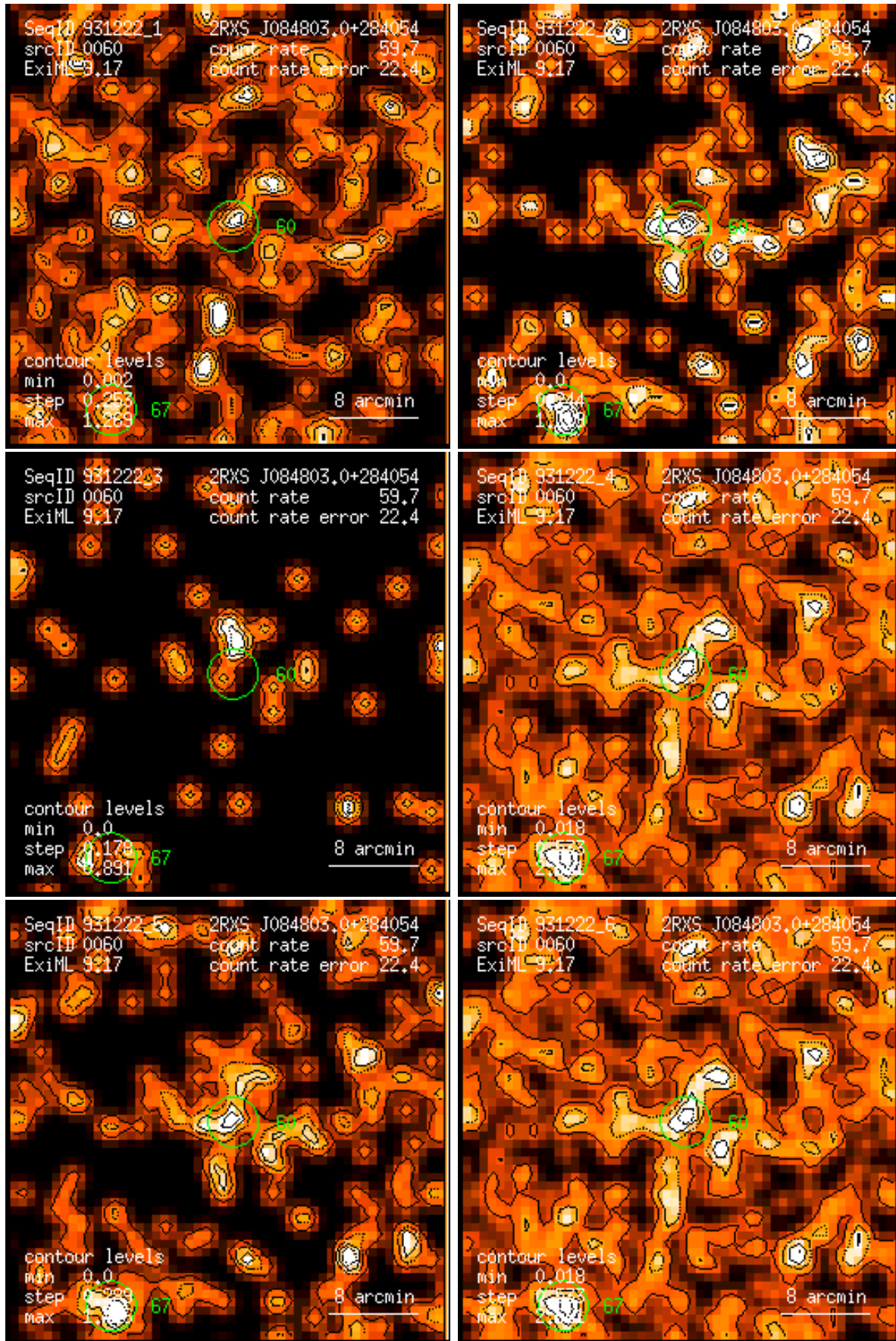
Figure 60: RASS 931222: detection 0060: band rate images, Gaussian filter: (1) PSPC channels 11 – 41, (2) 52 – 90, (3) 91 – 201, (4) 11 – 235, (5) 52 – 201, (6) 11 – 201. Broad band rates in counts/ks. Band rate contour levels in counts/ks/arcmin 2 .
