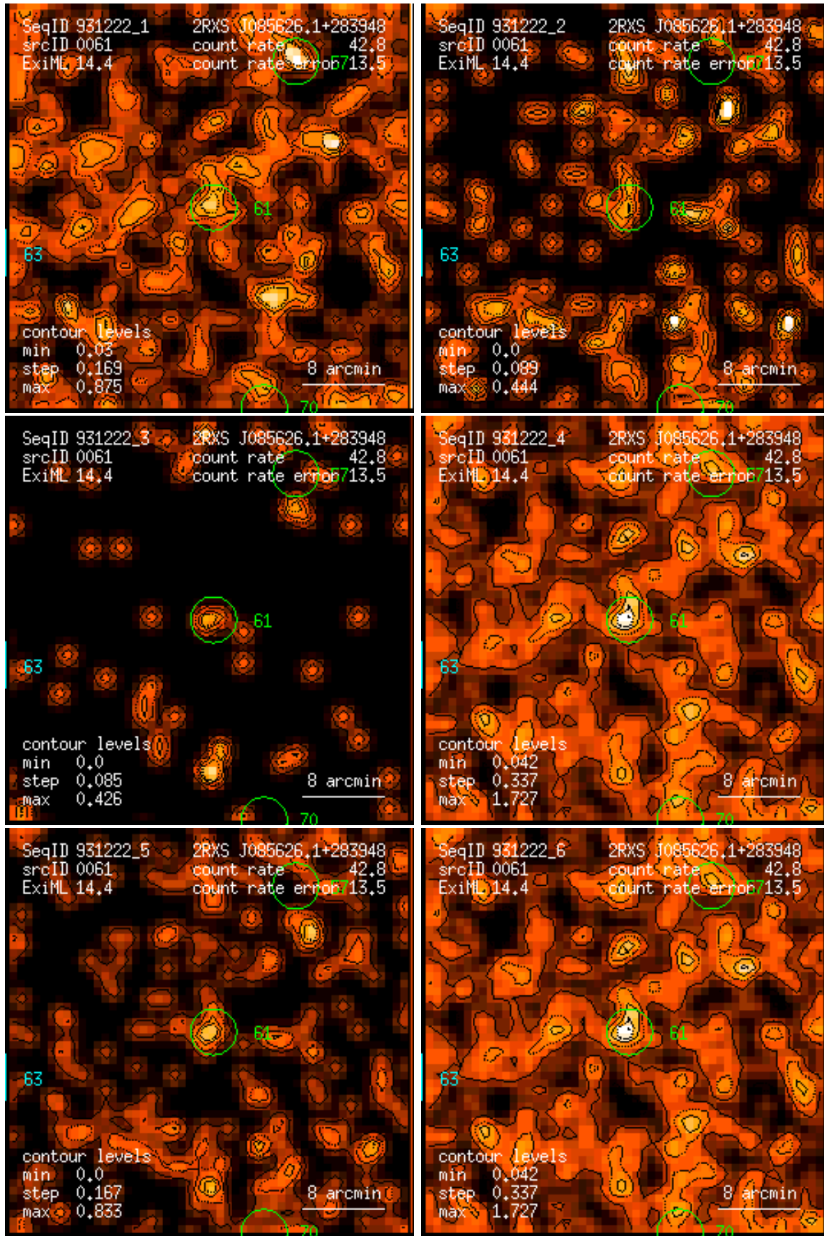
Figure 61: RASS 931222: detection 0061: band rate images, Gaussian filter: (1) PSPC channels 11 – 41, (2) 52 – 90, (3) 91 – 201, (4) 11 – 235, (5) 52 – 201, (6) 11 – 201. Broad band rates in counts/ks. Band rate contour levels in counts/ks/arcmin 2 .
