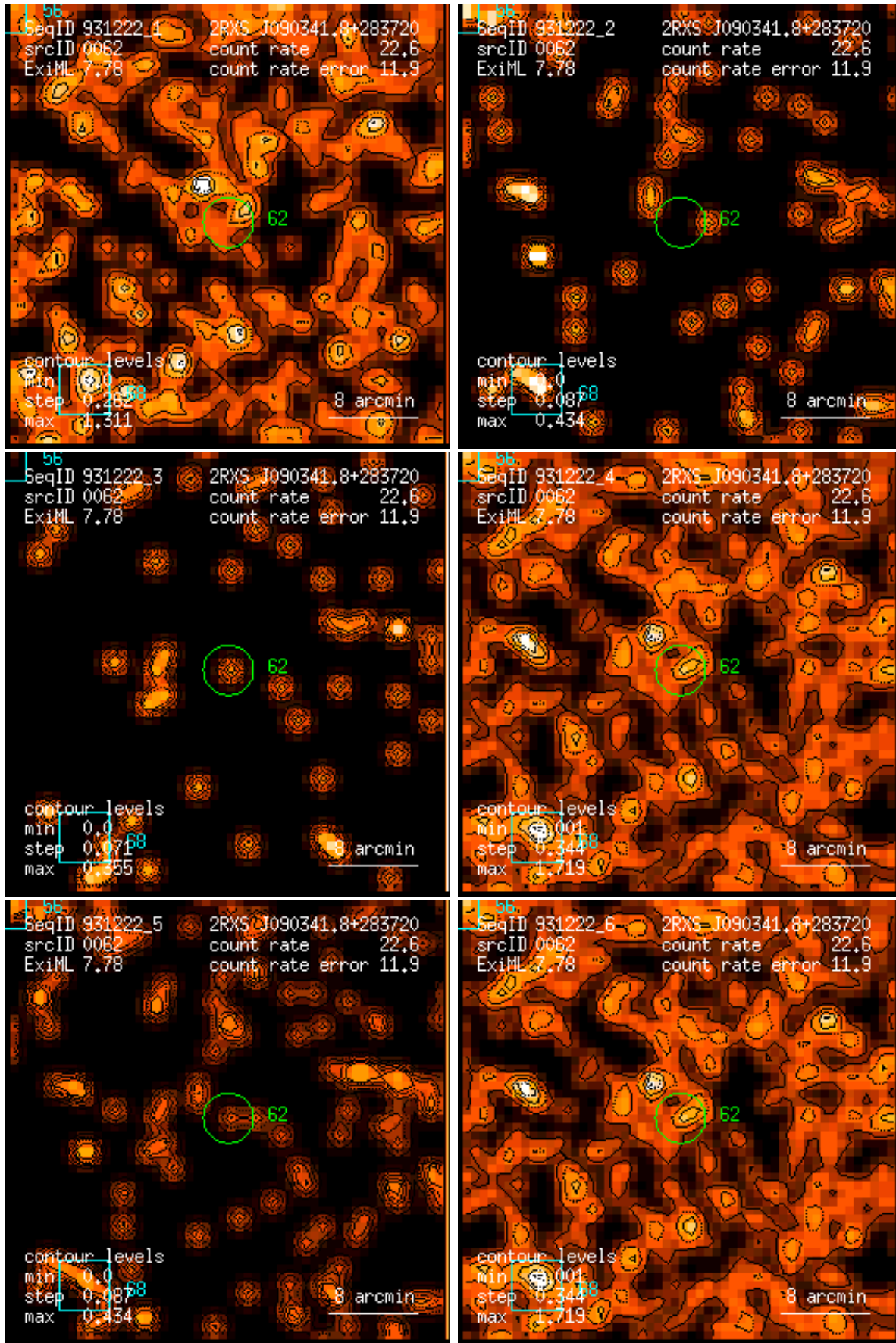
Figure 62: RASS 931222: detection 0062: band rate images, Gaussian filter: (1) PSPC channels 11 – 41, (2) 52 – 90, (3) 91 – 201, (4) 11 – 235, (5) 52 – 201, (6) 11 – 201. Broad band rates in counts/ks. Band rate contour levels in counts/ks/arcmin 2 .
