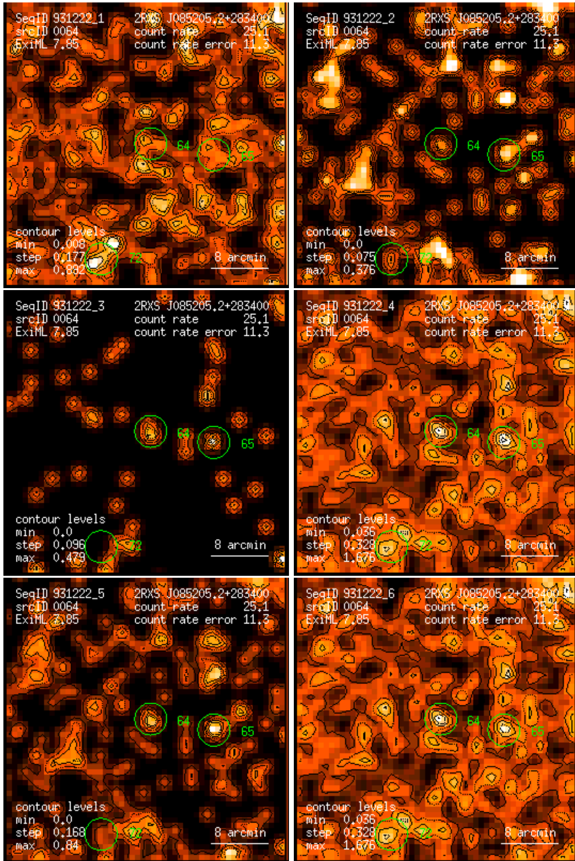
Figure 64: RASS 931222: detection 0064: band rate images, Gaussian filter: (1) PSPC channels 11 – 41, (2) 52 – 90, (3) 91 – 201, (4) 11 – 235, (5) 52 – 201, (6) 11 – 201. Broad band rates in counts/ks. Band rate contour levels in counts/ks/arcmin 2 .
