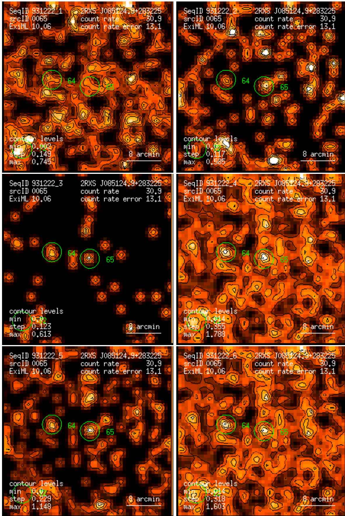
Figure 65: RASS 931222: detection 0065: band rate images, Gaussian filter: (1) PSPC channels 11 – 41, (2) 52 – 90, (3) 91 – 201, (4) 11 – 235, (5) 52 – 201, (6) 11 – 201. Broad band rates in counts/ks. Band rate contour levels in counts/ks/arcmin 2 .
