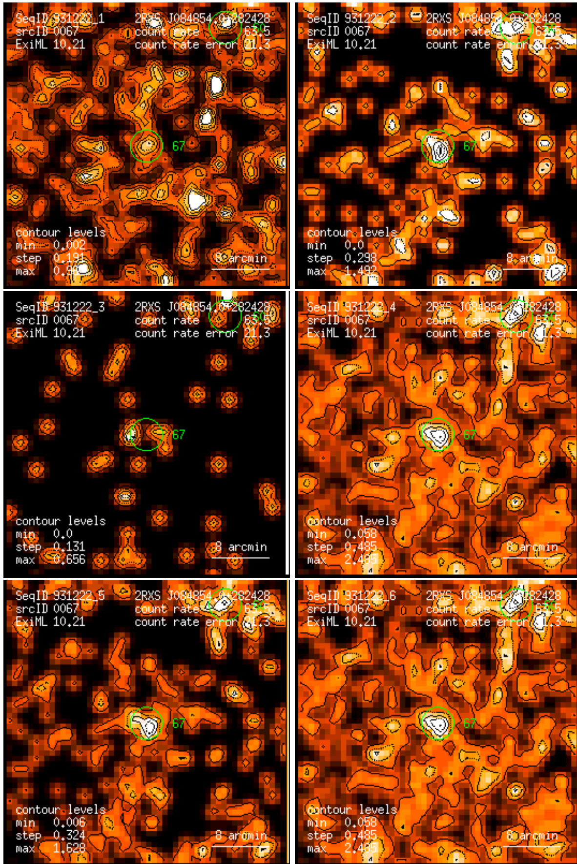
Figure 67: RASS 931222: detection 0067: band rate images, Gaussian filter: (1) PSPC channels 11 – 41, (2) 52 – 90, (3) 91 – 201, (4) 11 – 235, (5) 52 – 201, (6) 11 – 201. Broad band rates in counts/ks. Band rate contour levels in counts/ks/arcmin 2 .
