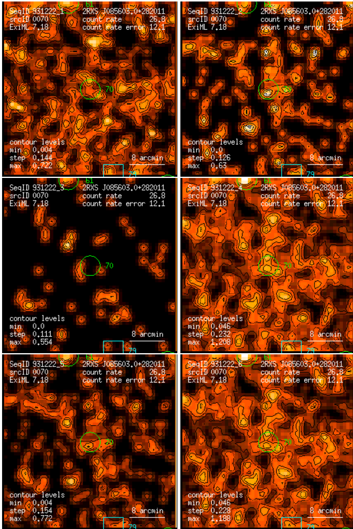
Figure 70: RASS 931222: detection 0070: band rate images, Gaussian filter: (1) PSPC channels 11 – 41, (2) 52 – 90, (3) 91 – 201, (4) 11 – 235, (5) 52 – 201, (6) 11 – 201. Broad band rates in counts/ks. Band rate contour levels in counts/ks/arcmin 2 .
