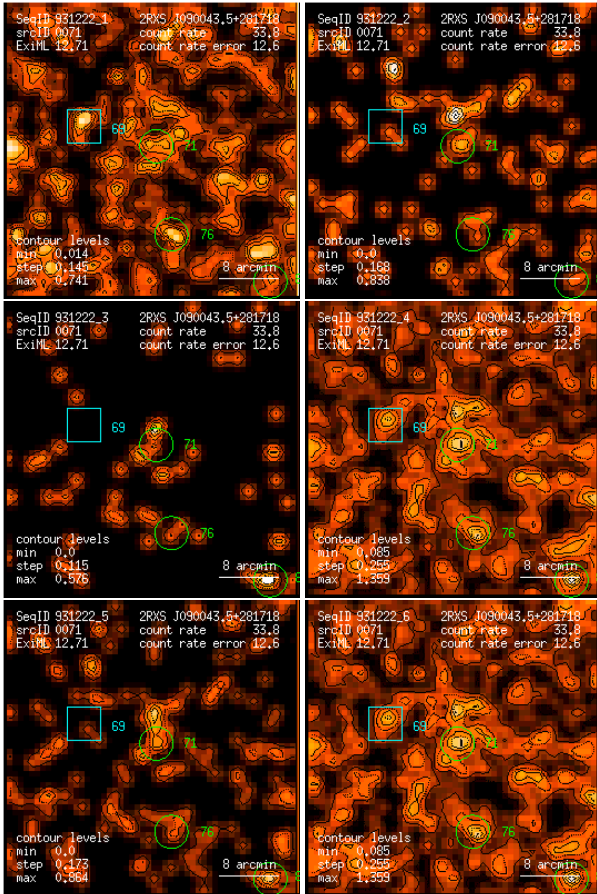
Figure 71: RASS 931222: detection 0071: band rate images, Gaussian filter: (1) PSPC channels 11 – 41, (2) 52 – 90, (3) 91 – 201, (4) 11 – 235, (5) 52 – 201, (6) 11 – 201. Broad band rates in counts/ks. Band rate contour levels in counts/ks/arcmin 2 .
