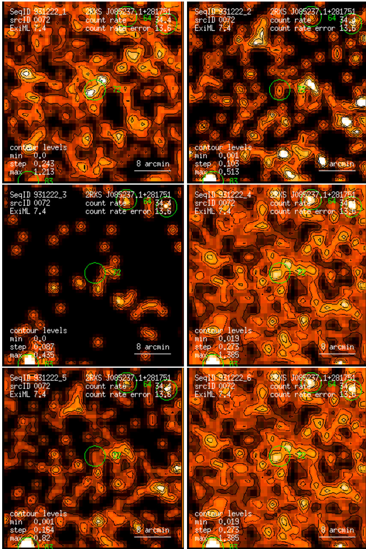
Figure 72: RASS 931222: detection 0072: band rate images, Gaussian filter: (1) PSPC channels 11 – 41, (2) 52 – 90, (3) 91 – 201, (4) 11 – 235, (5) 52 – 201, (6) 11 – 201. Broad band rates in counts/ks. Band rate contour levels in counts/ks/arcmin 2 .
