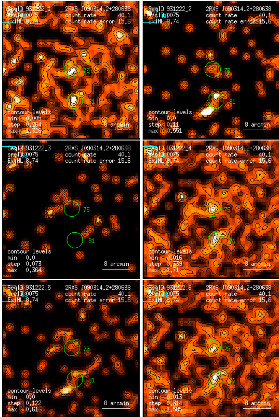
Figure 75: RASS 931222: detection 0075: band rate images, Gaussian filter: (1) PSPC channels 11 – 41, (2) 52 – 90, (3) 91 – 201, (4) 11 – 235, (5) 52 – 201, (6) 11 – 201. Broad band rates in counts/ks. Band rate contour levels in counts/ks/arcmin 2 .
